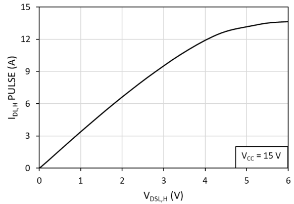
Fig. 6. Pulsed Drain current ( I_{D_{SL,H}} \text{ PULSE} ) vs. drain-to-source voltage ( V_{D_{SL,H}} ) at T = 125\text{ }^\circ\text{C}
