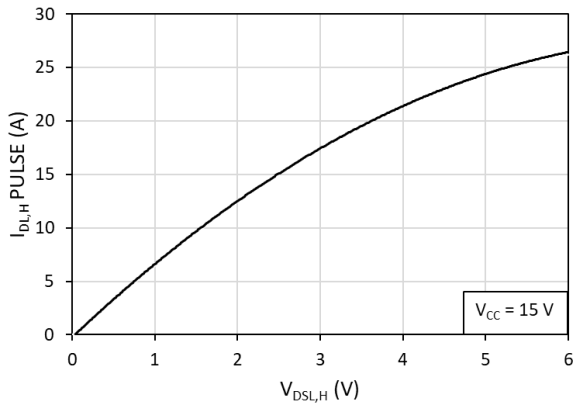
Fig. 5. Pulsed Drain current ( I_{D_{SL,H}} \text{ PULSE} ) vs. drain-to-source voltage ( V_{D_{SL,H}} ) at T = 25\text{ }^\circ\text{C}
