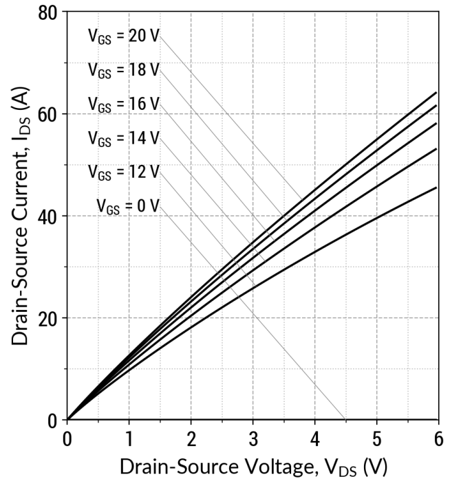
Figure 2: Output Characteristics ( T_j = 150^\circ\text{C} )
