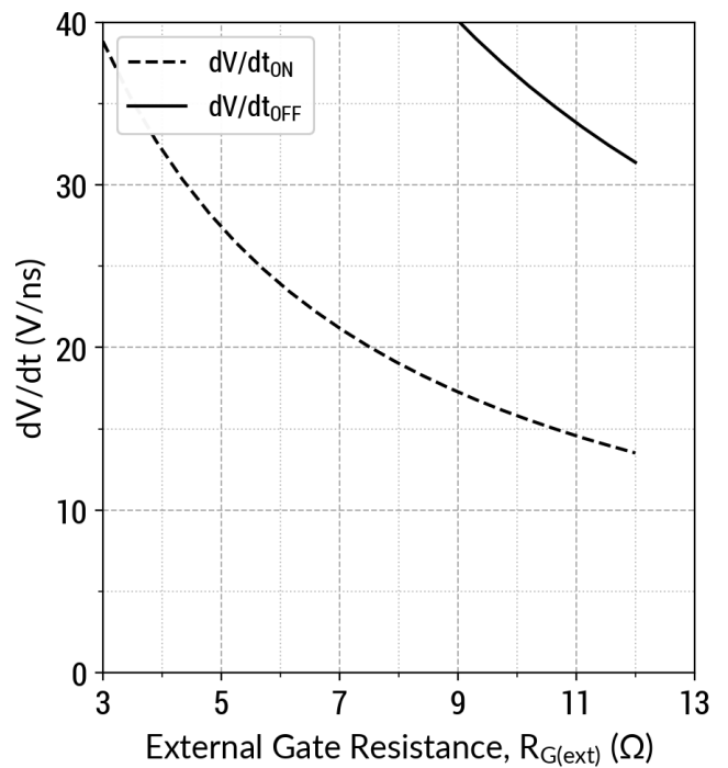
Figure 26: dV/dt v/s R_{G(ext)} ( V_{DD} = 1700V )
