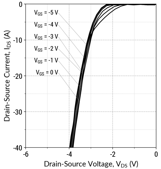
Figure 18: Body Diode Characteristics ( T_j = 150^\circ\text{C} )
