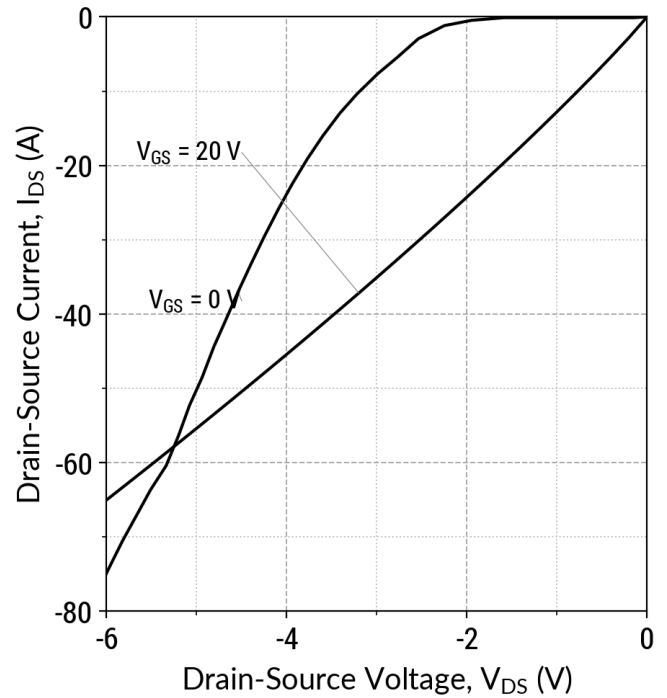
Figure 20: Third Quadrant Characteristics ( T_j = 150^\circ\text{C} )
