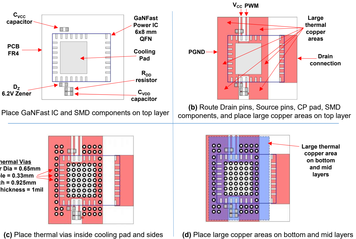
Fig 2. GaNFast IC PCB layout steps (without CS resistors)
